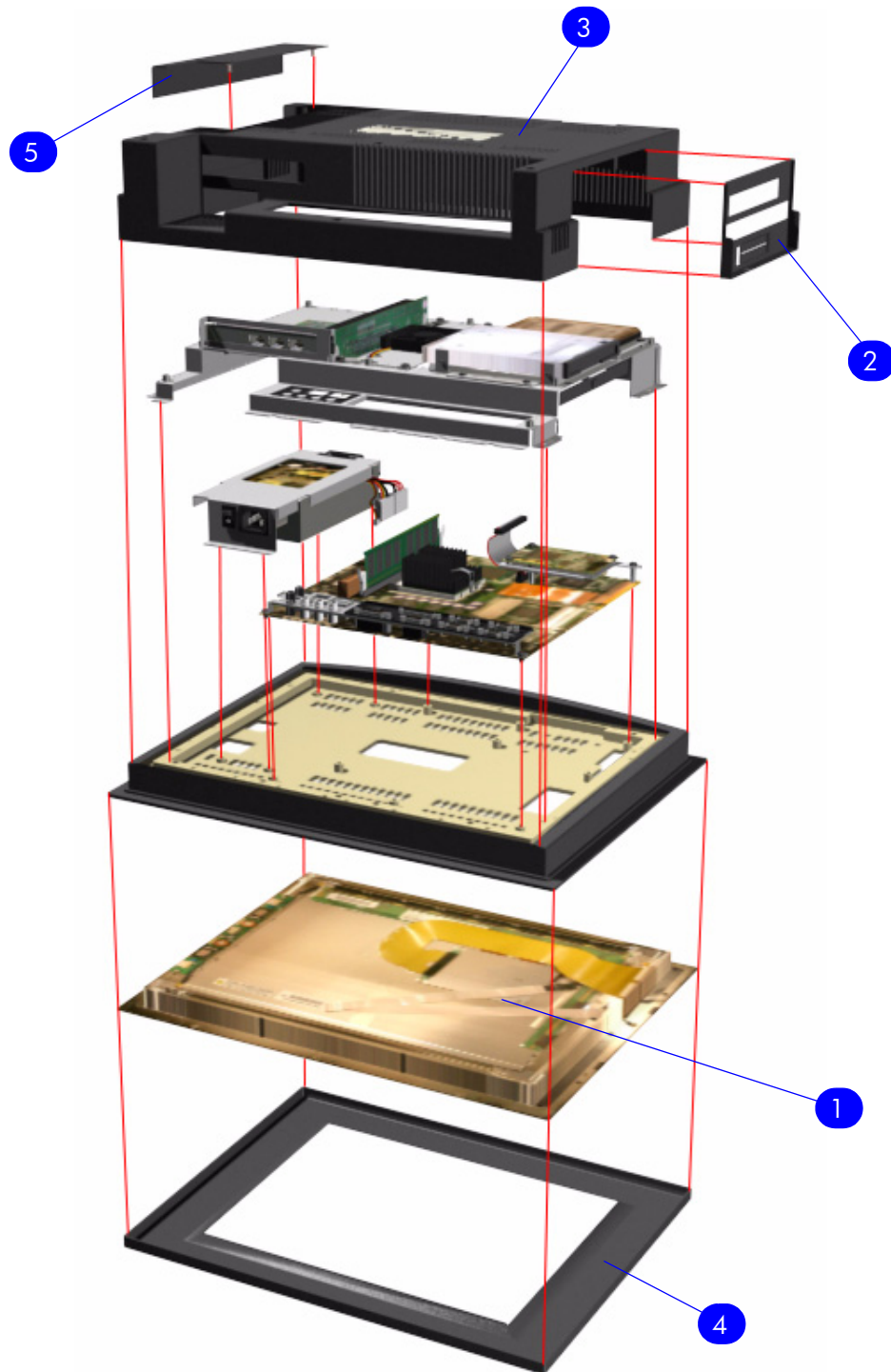
Figure 11: Touch Screen Components (Part 1)
