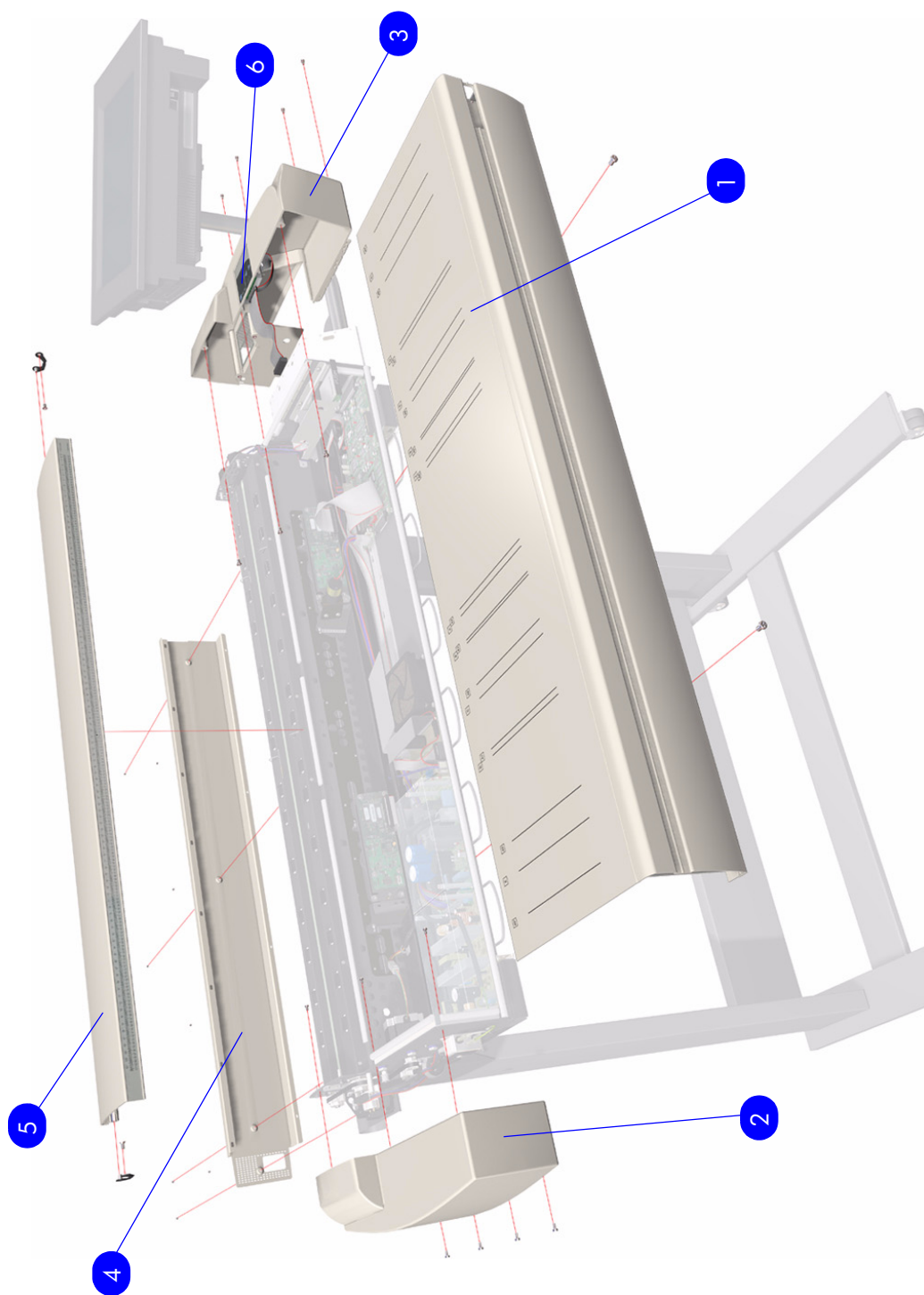
Figure 4: Copier Covers
