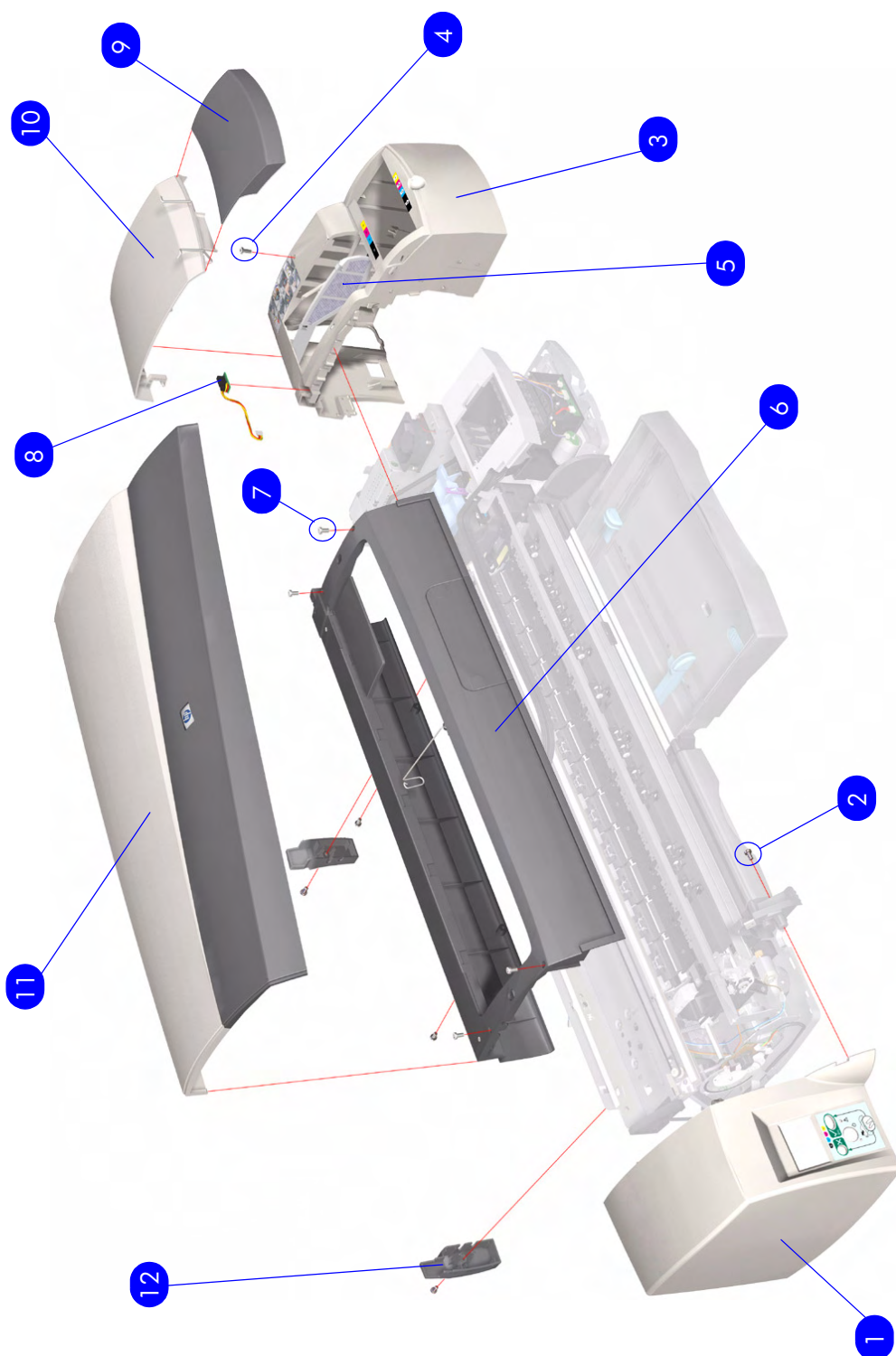
Figure 1: Cover Assemblies
