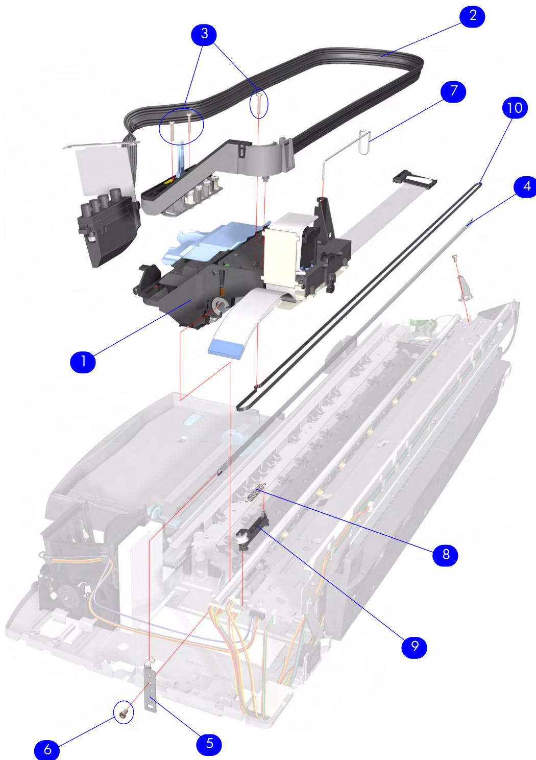
Figure 5: Scan-Axis Assemblies
