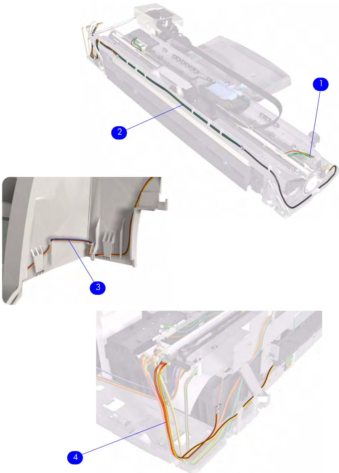
Figure 10: Cable Harnesses
