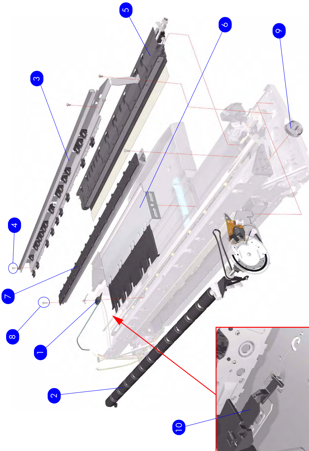
Figure 6: Top Paper Path Assemblies
