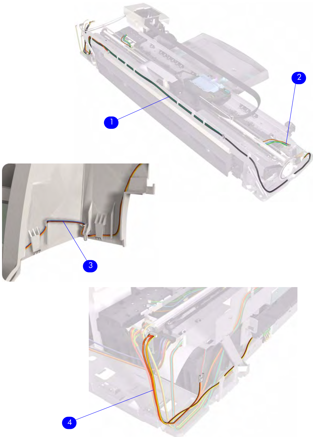
Figure 9: Cable Harnesses
