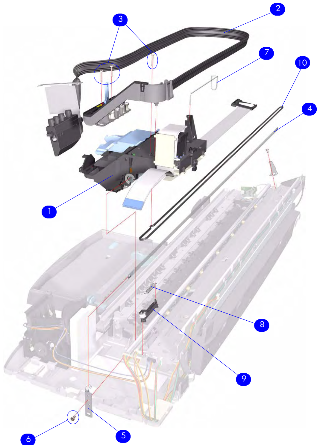
Figure 5: Scan-Axis Assemblies
