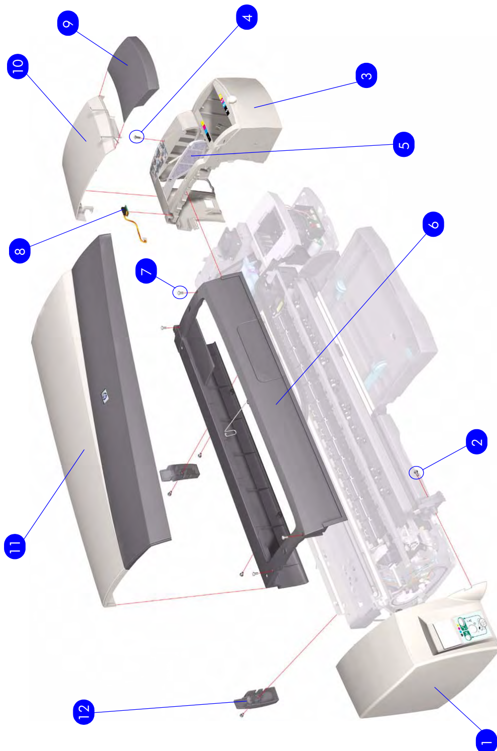
Figure 1: Cover Assemblies
