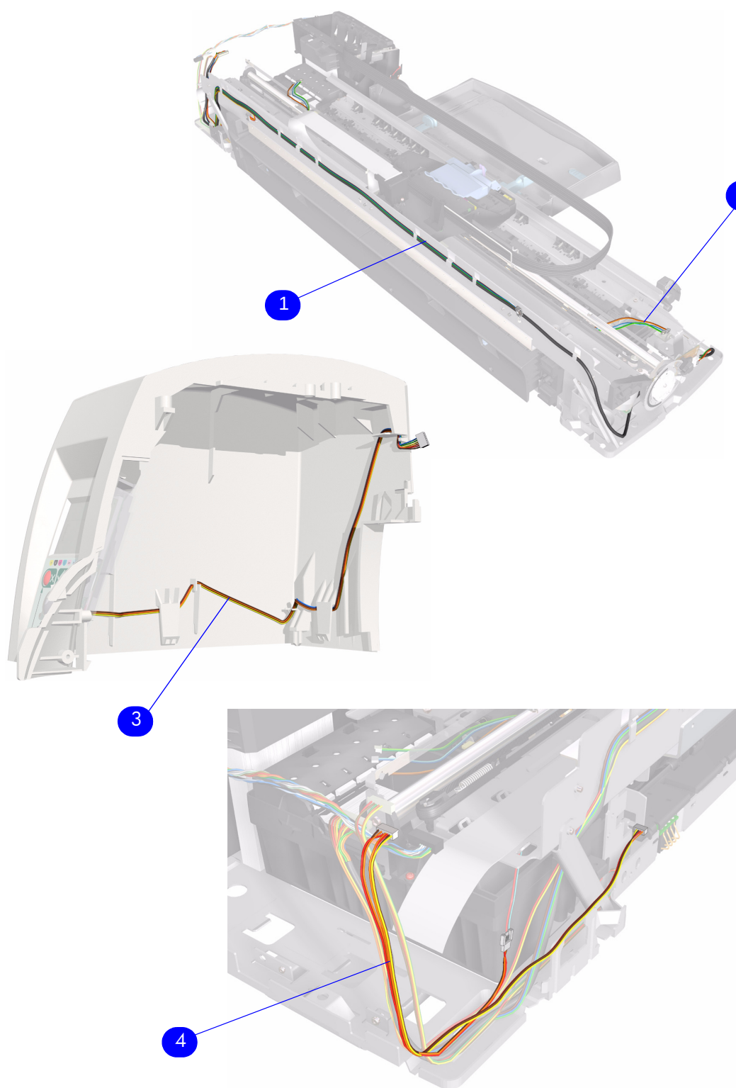
Figure 11: Cable Harnesses
