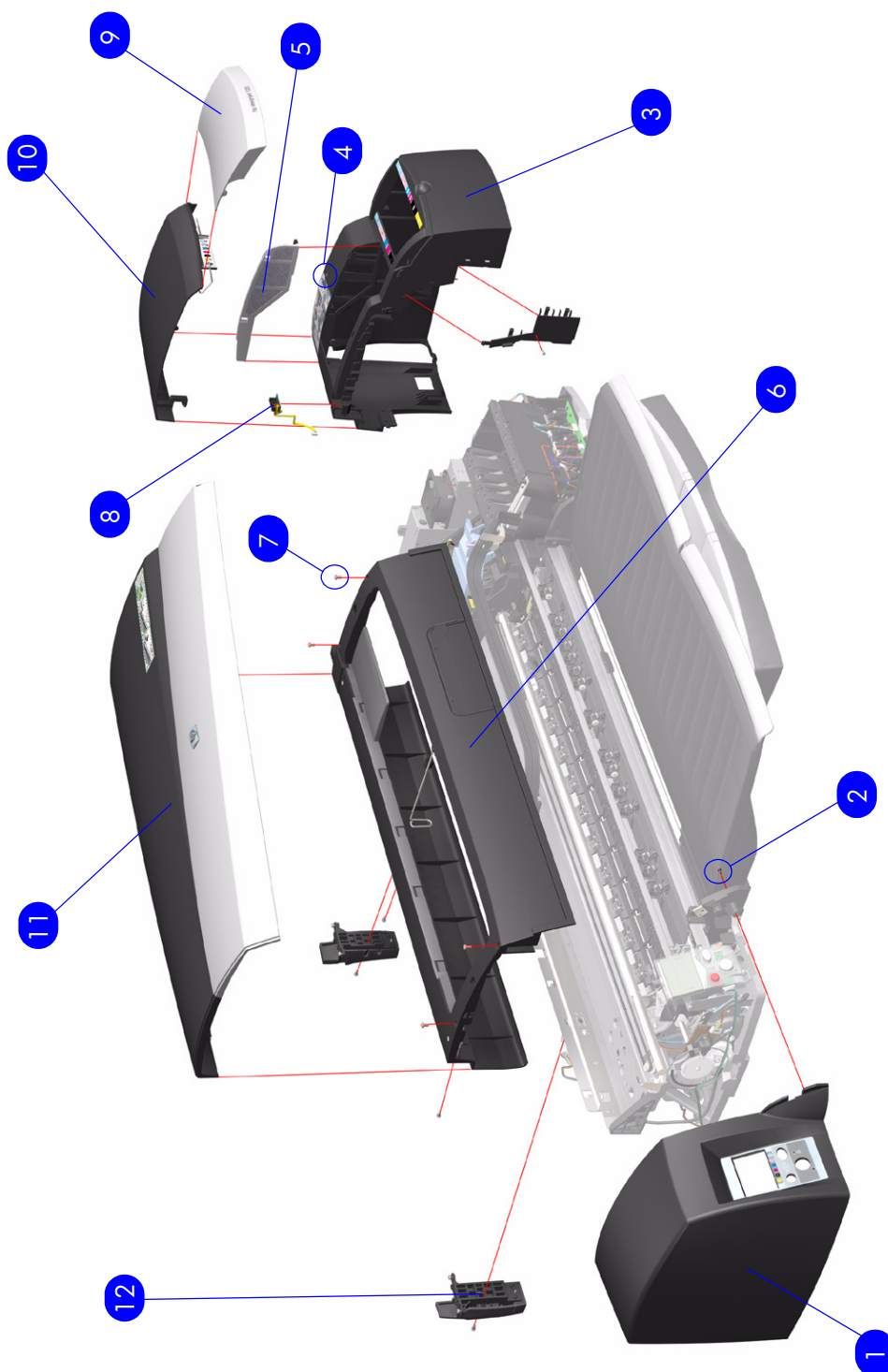
Figure 2: Cover Assemblies (Applicable to DesignJet 130/130nr)
