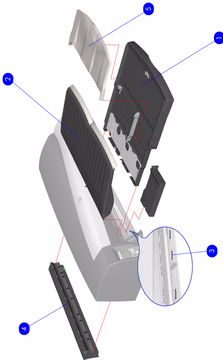
Figure 10: Paper Feed Assemblies (Applicable to DesignJet 130/130nr)
