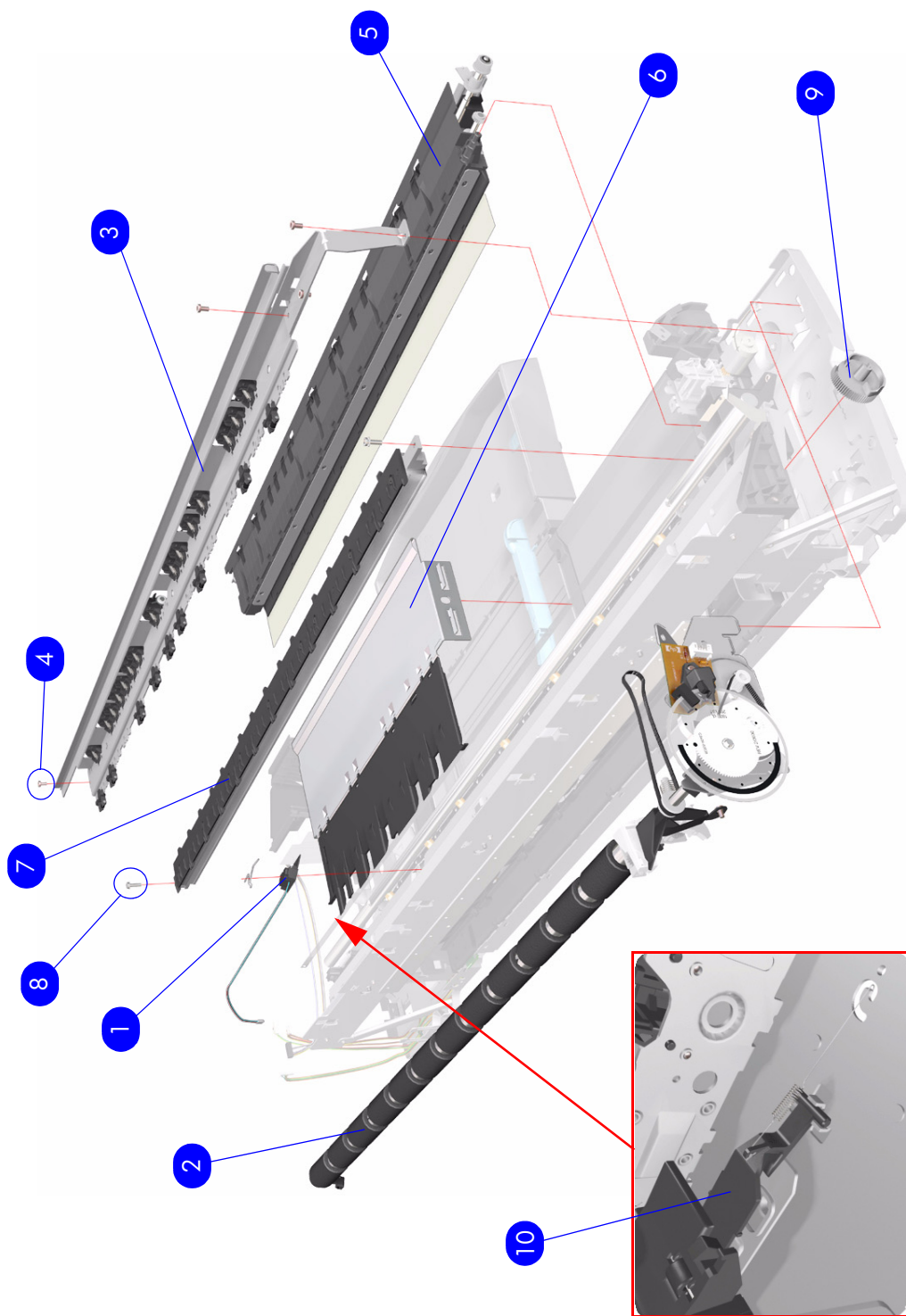
Figure 7: Top Paper Path Assemblies
