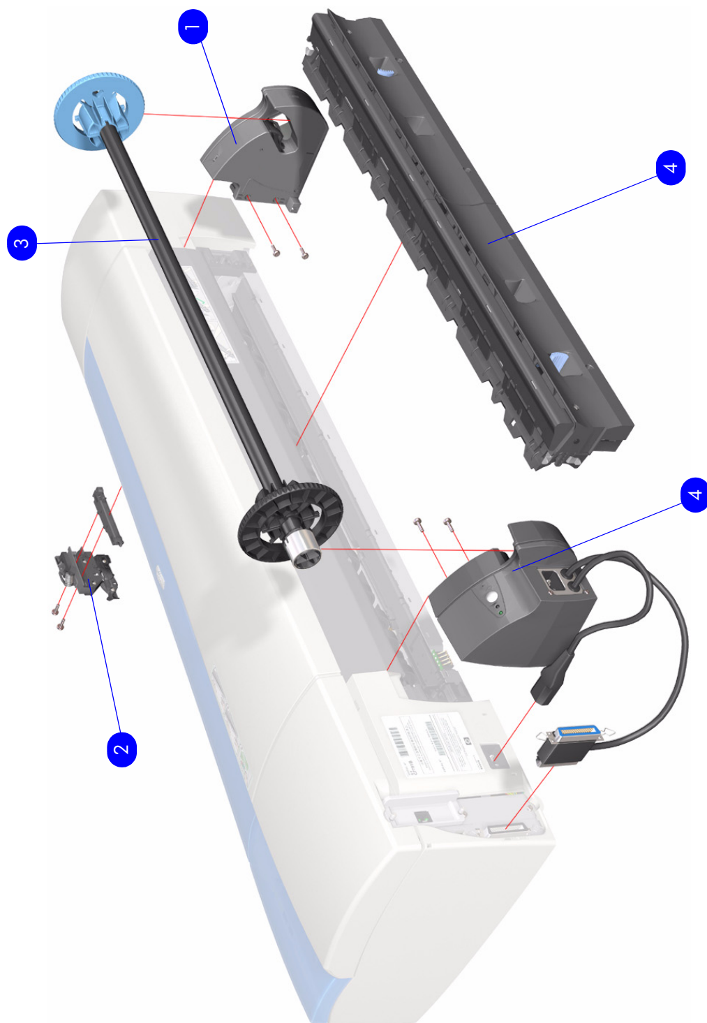
Figure 15: Rollfeed Components
