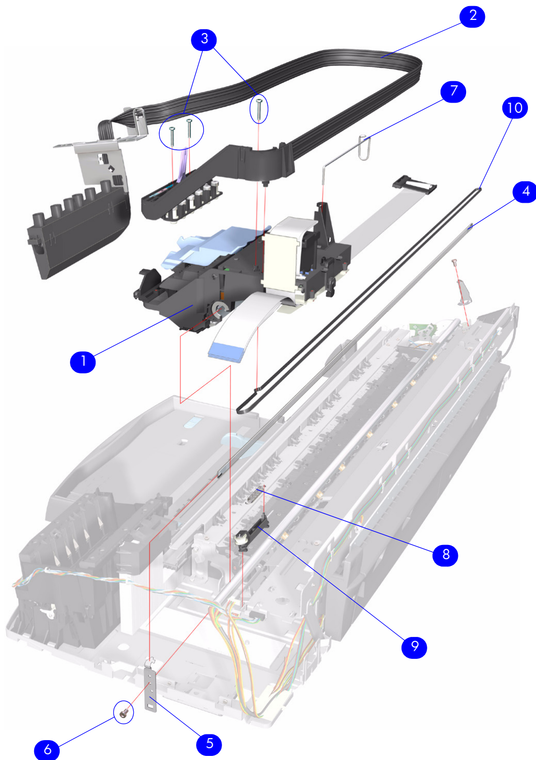
Figure 6: Scan-Axis Assemblies
