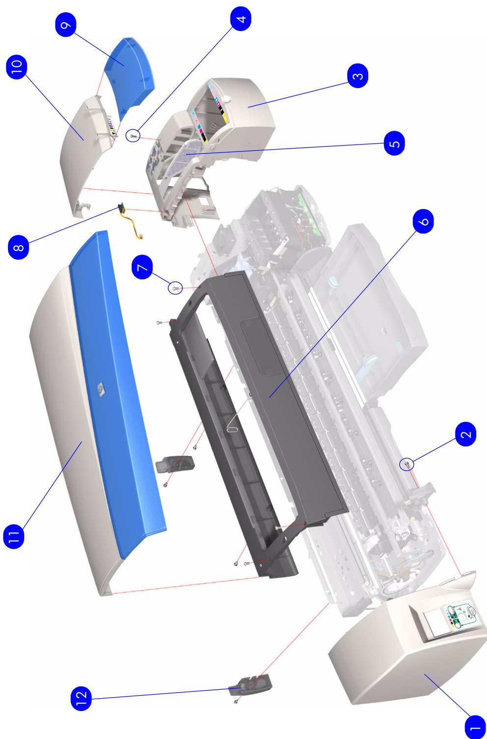
Figure 1: Cover Assemblies (Applicable to DesignJet 120/120nr)
