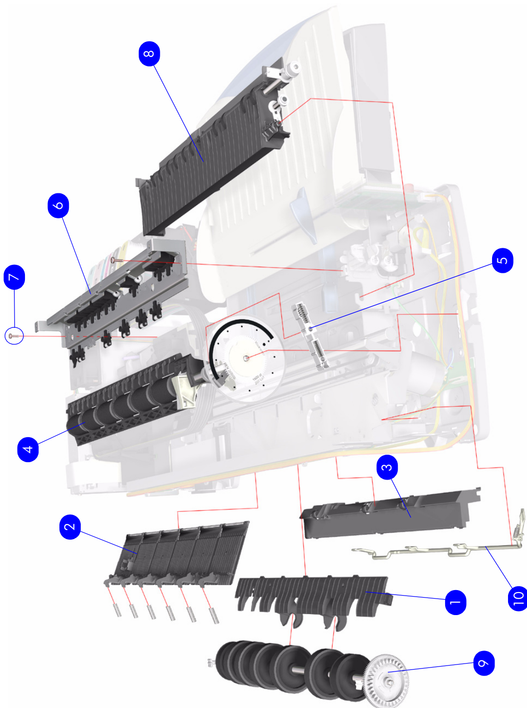
Figure 7: Paper Path Assemblies
