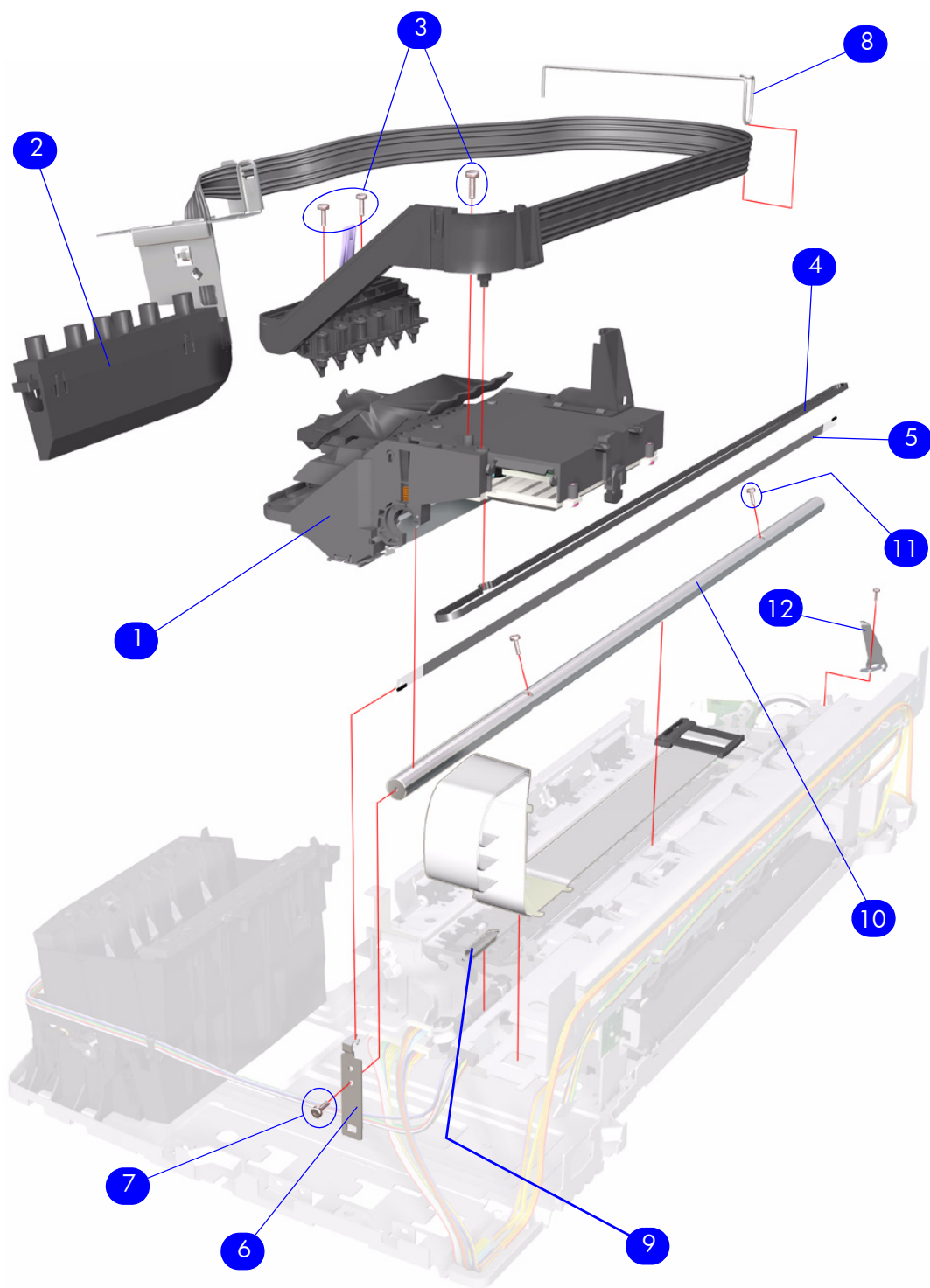
Figure 6: Scan-Axis Assemblies
