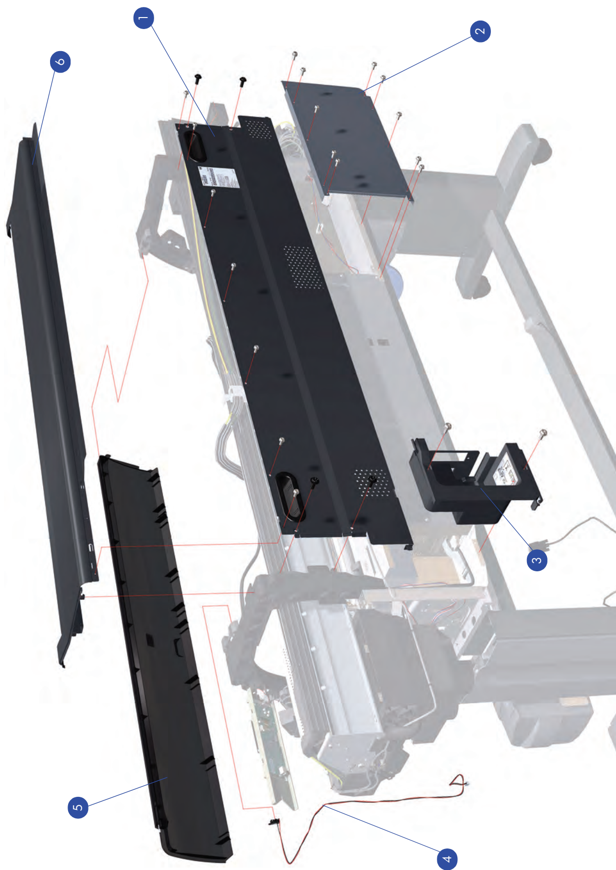
Figure 2: Center Covers
