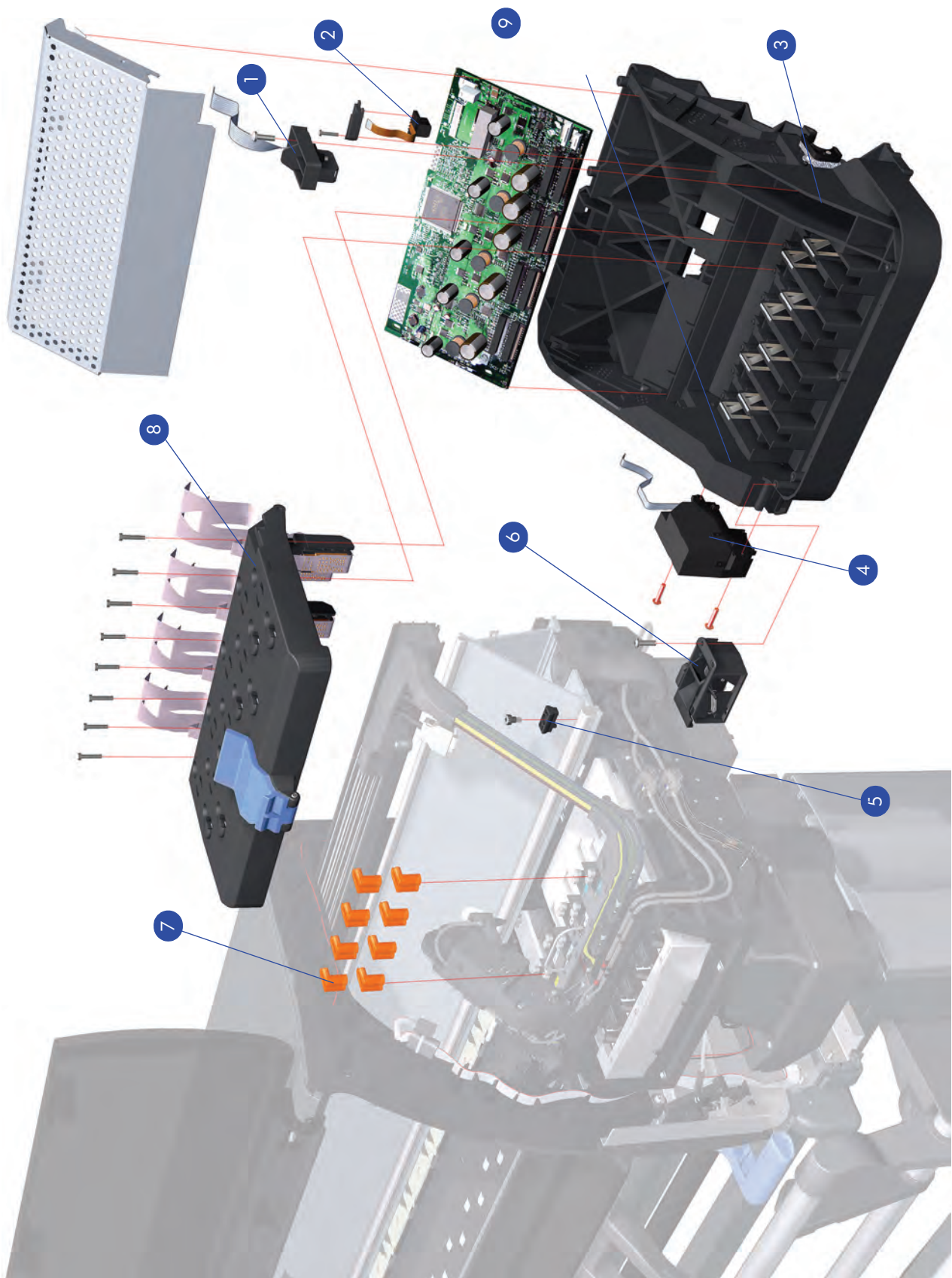
Figure 8: Carriage Assembly
