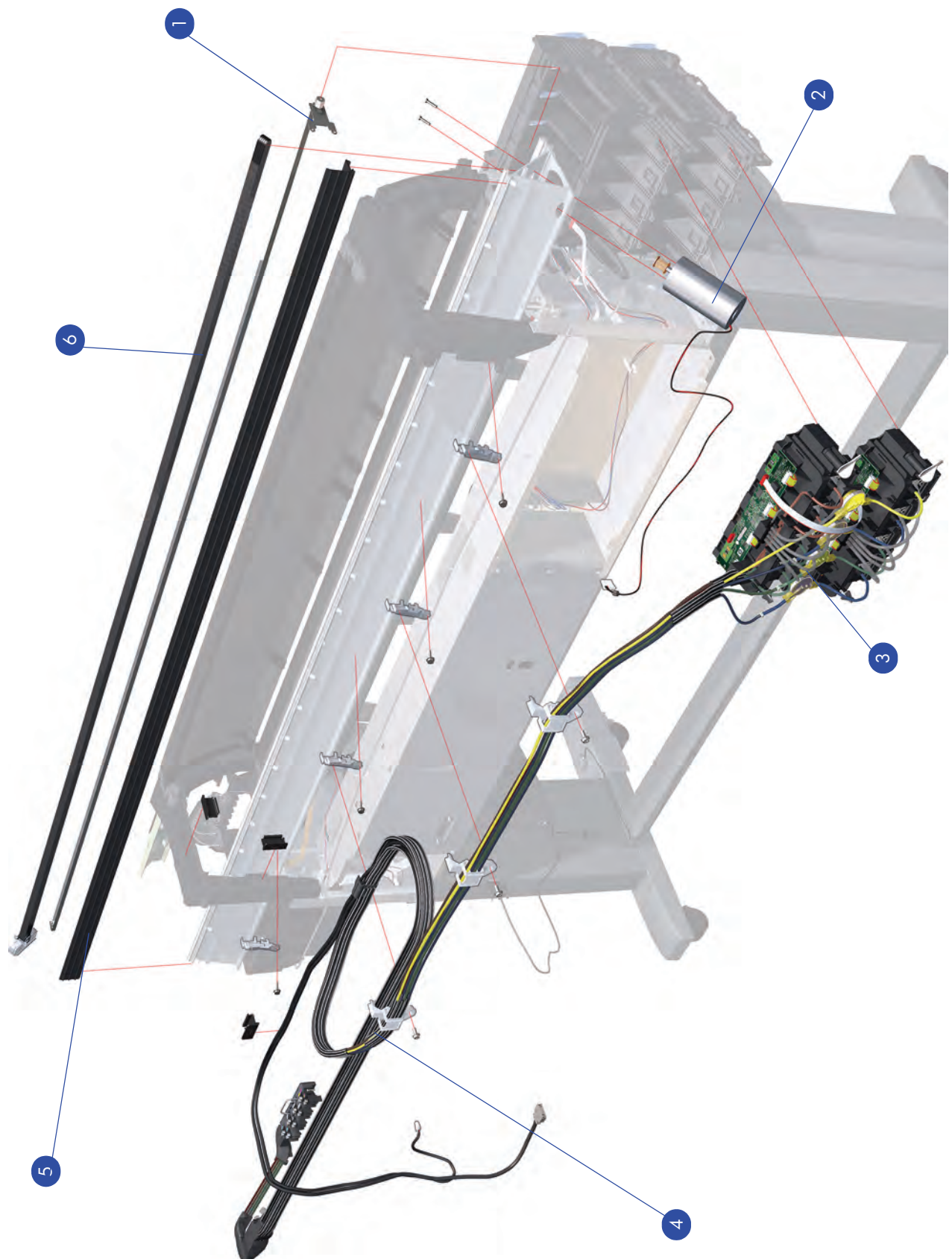
Figure 9: Scan-Axis Assemblies
