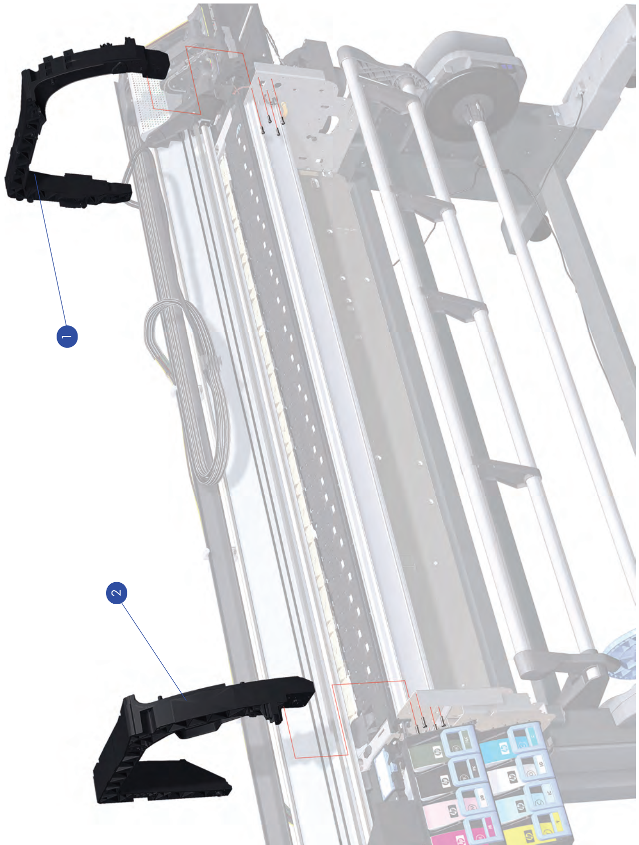
Figure 15: Arc Assemblies
