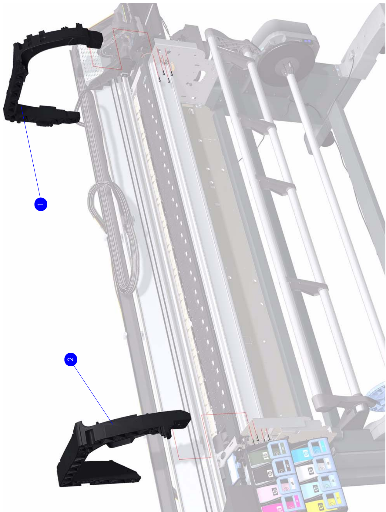
Figure 15: Arc Assemblies
