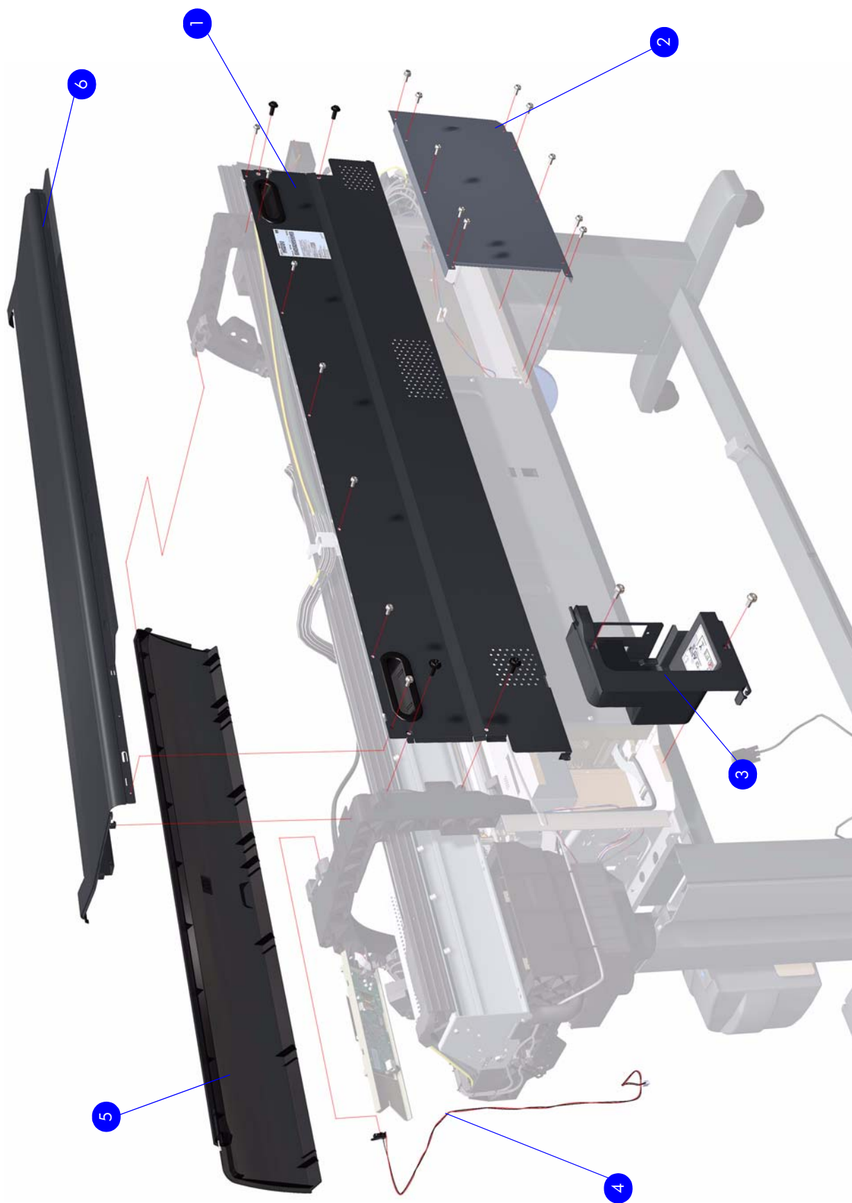
Figure 2: Center Covers
