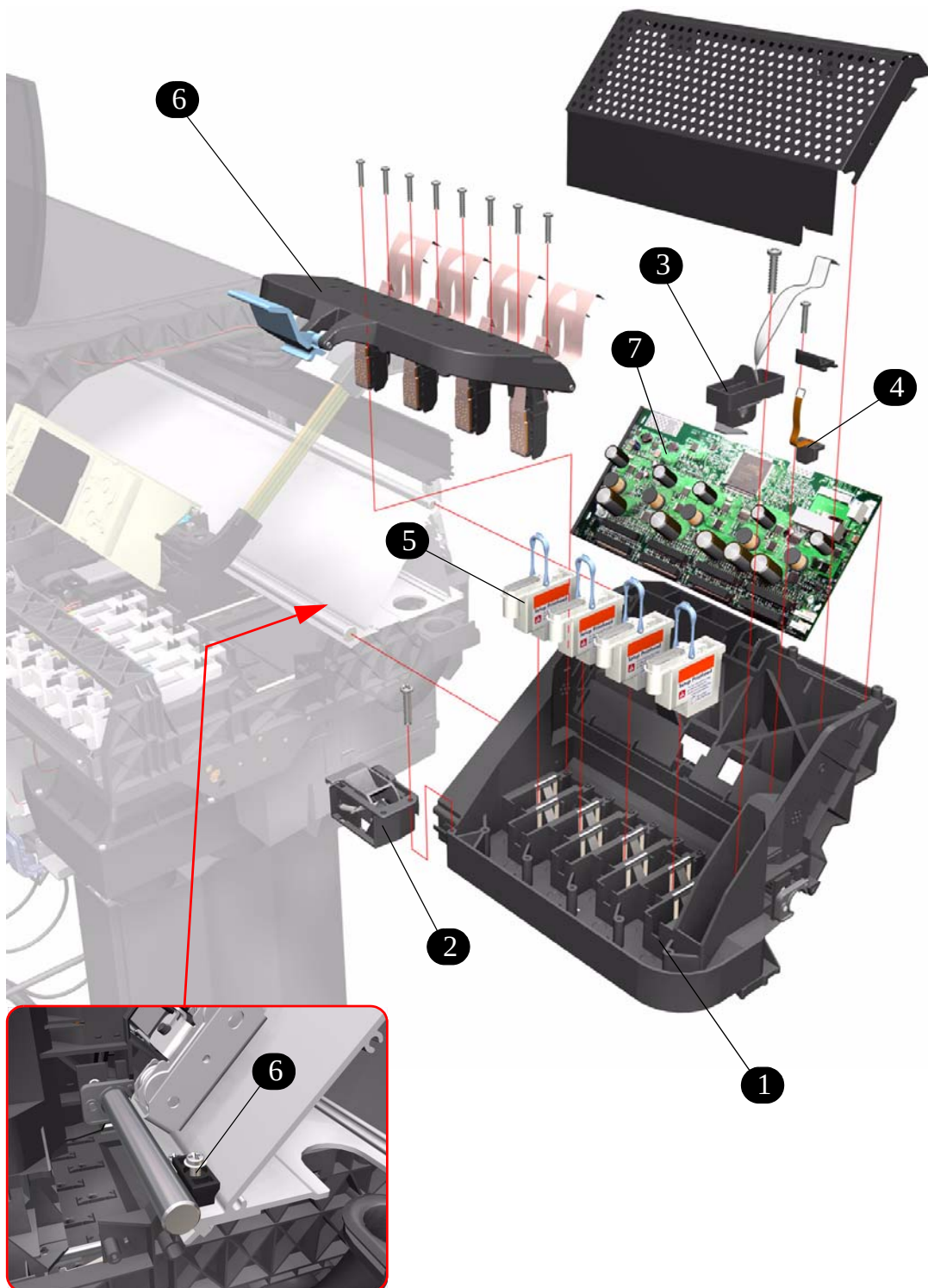
Figure 8: Carriage Assembly
