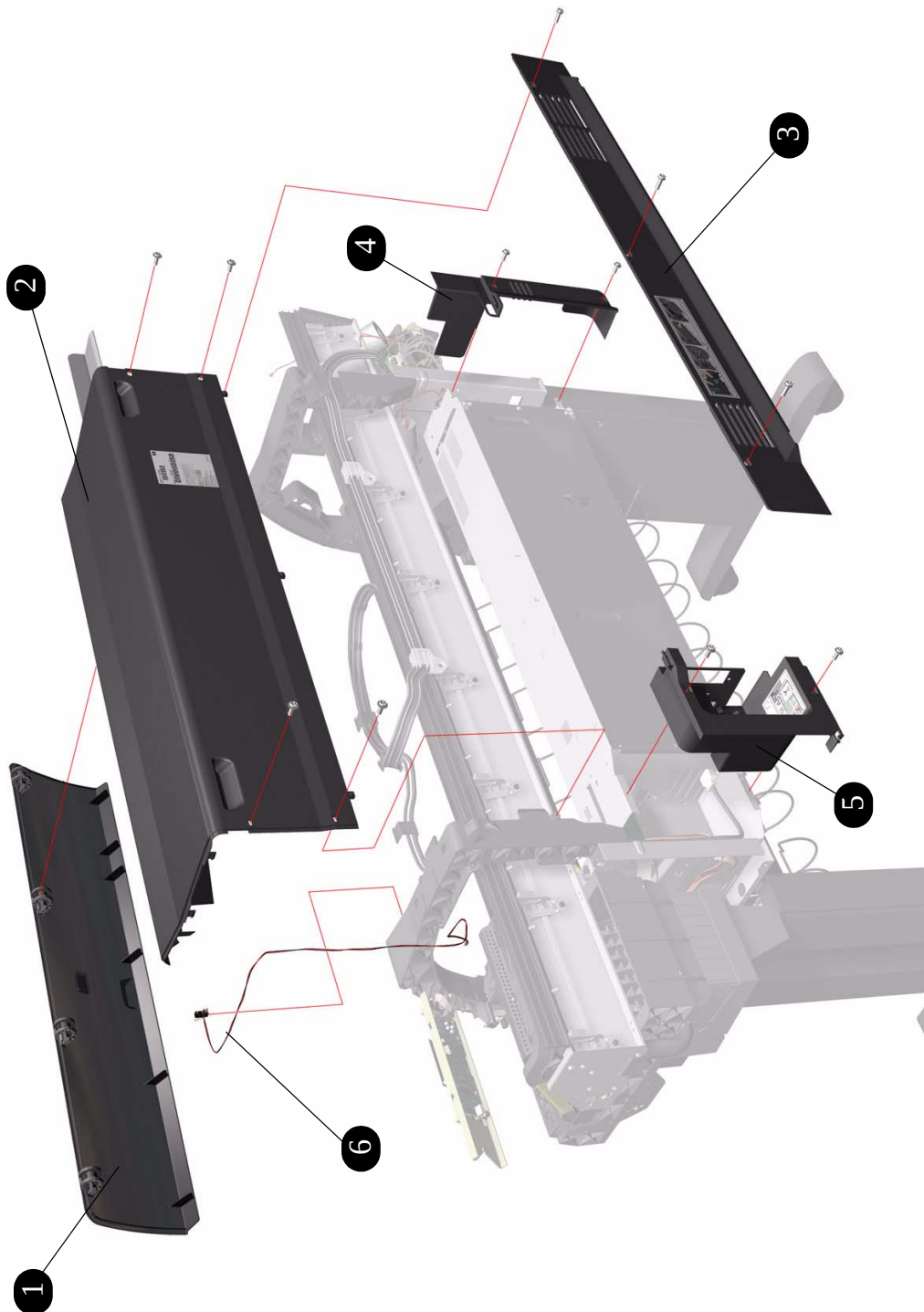
Figure 2: Center Covers
