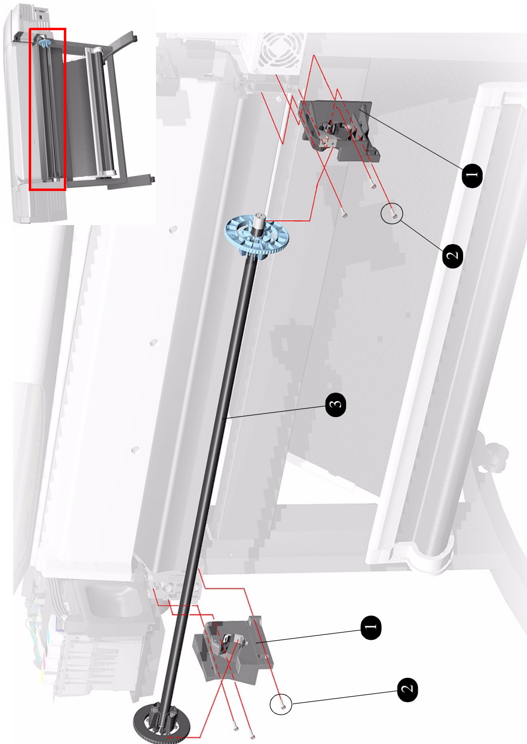
Figure 5: Rollfeed Module
