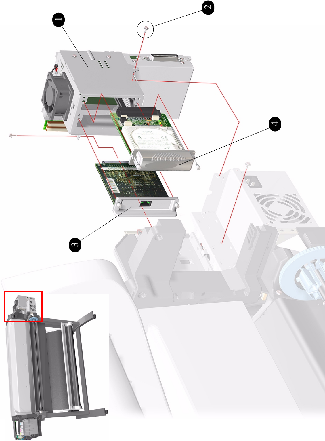
Figure 7: Electronics Module
