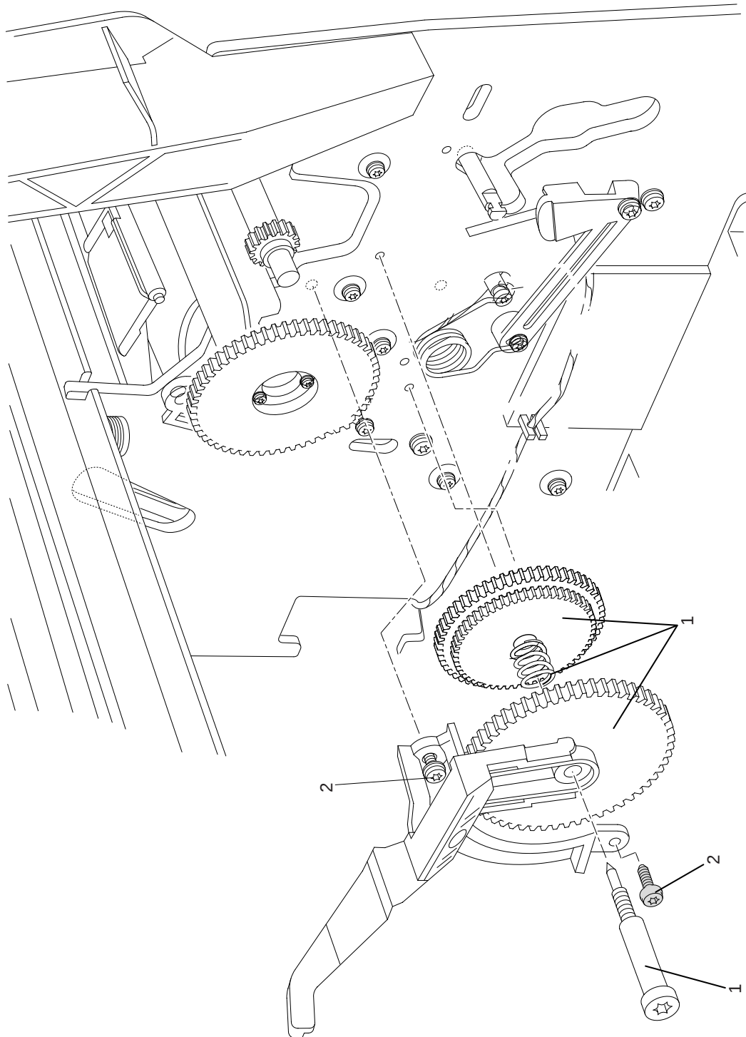
Figura 10: "Clutch Assembly"
