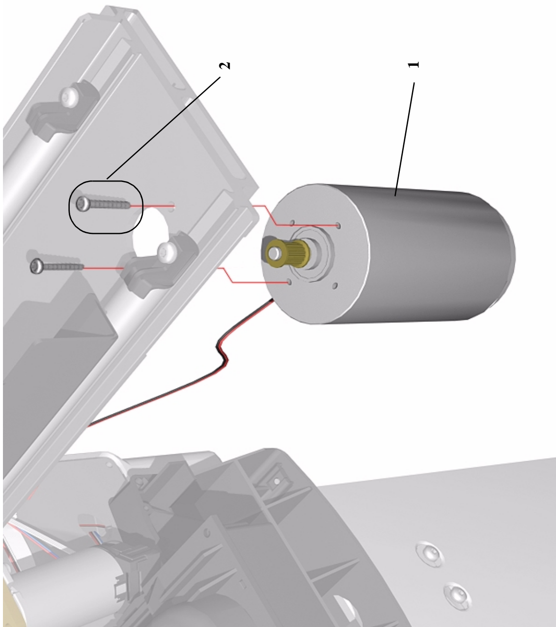
Figure 12: Scan-Axis Motor
